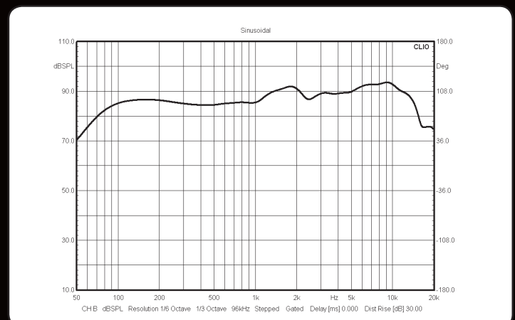
DLS SCANDINAVIA 3 FREQUENCY RESPONSE CURVE
