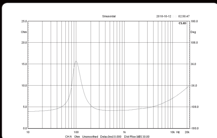
DLS SCANDINAVIA 3 IMPEDANCE CURVE
